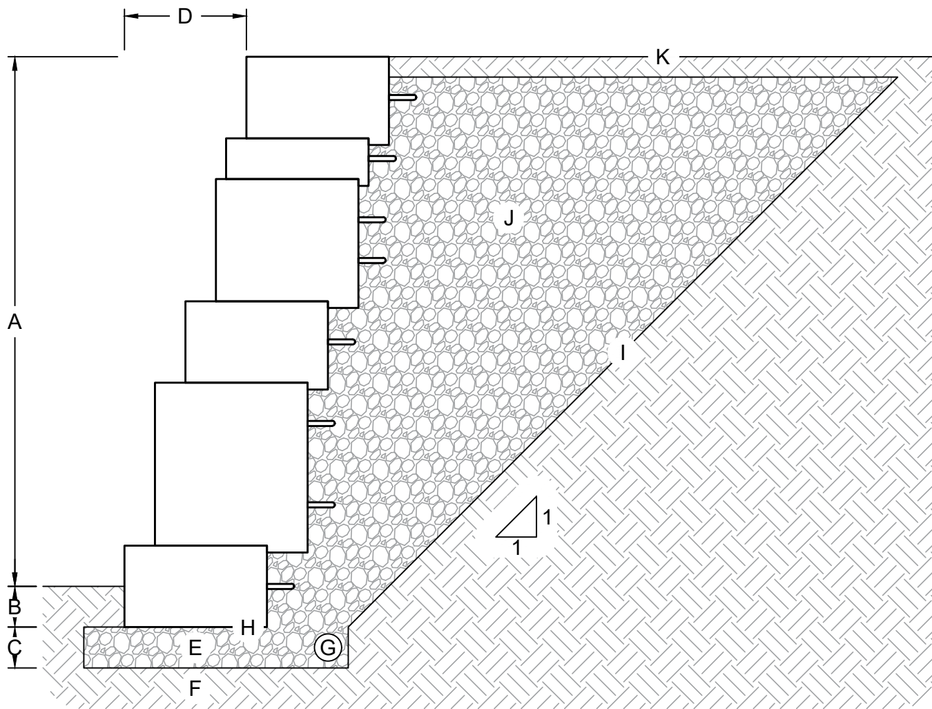
TYPICAL GRAVITY RETAINING WALL WITH AGGREGATE WEDGE BACKFILL TYPICAL INSTALLATION DETAILS
