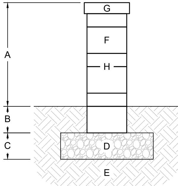
TYPICAL FREESTANDING SECTION (NO SCALE)
