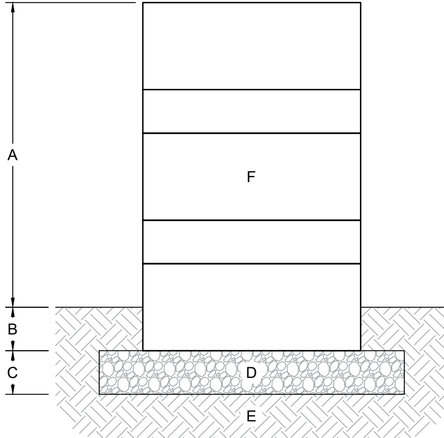
TYPICAL FREESTANDING WALL (NO SCALE)
